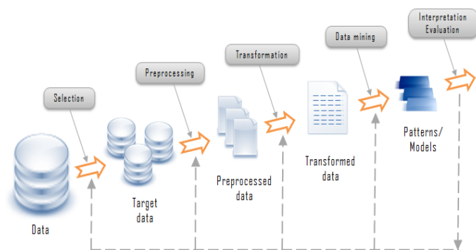
Fig.1:- Knowledge Discovery
