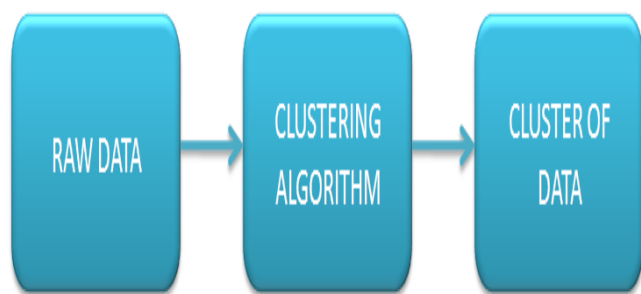
Fig.3:- Clustering
