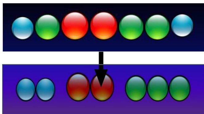
Fig.4:- Clustering
